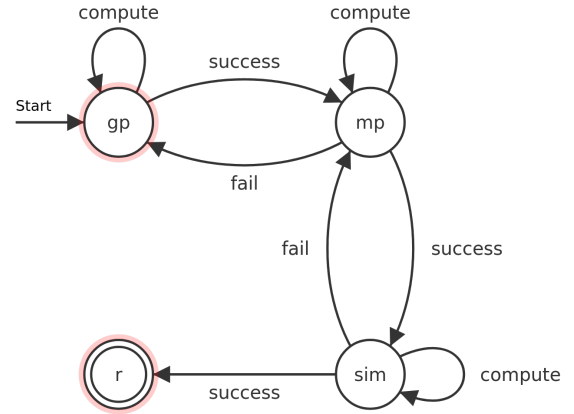
Figure 1: Finite state machine of the process for planning a movement for the robot
